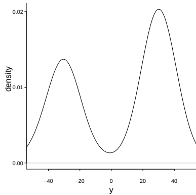
marginal density of y
