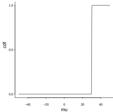
true CDF of \mu
