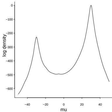
The true (unnormalized) log density of \mu
